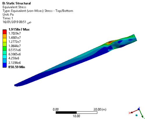
Figure 11: Von-Mises stress of Kevlar, rated speed
