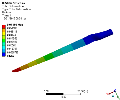
Figure 10: Total deformation of Kevlar, rated speed
