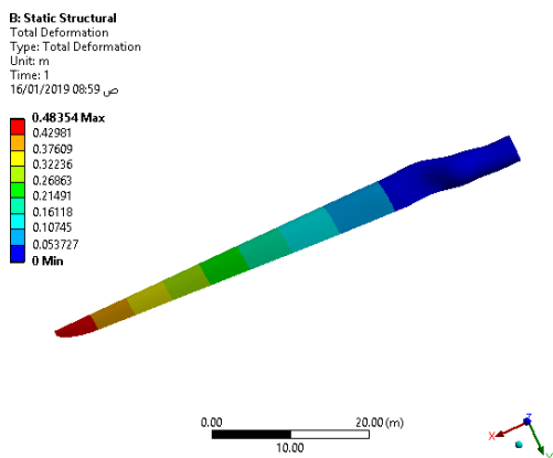
Figure 12: Total deformation of CFRP, rated speed
